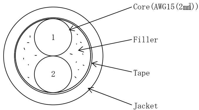
Cross-Section of Cable
